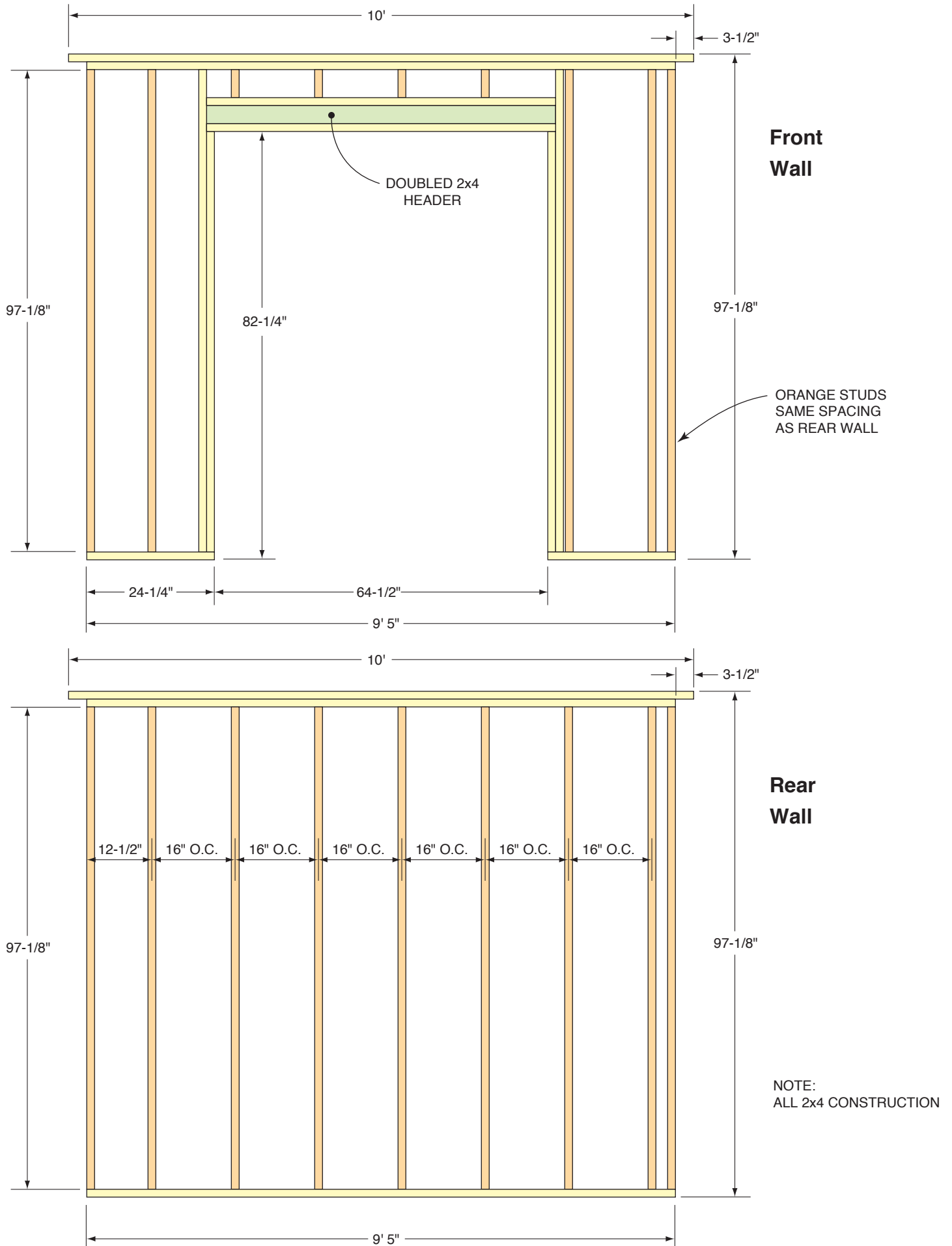
Figure E Framing the Front and Rear Walls
