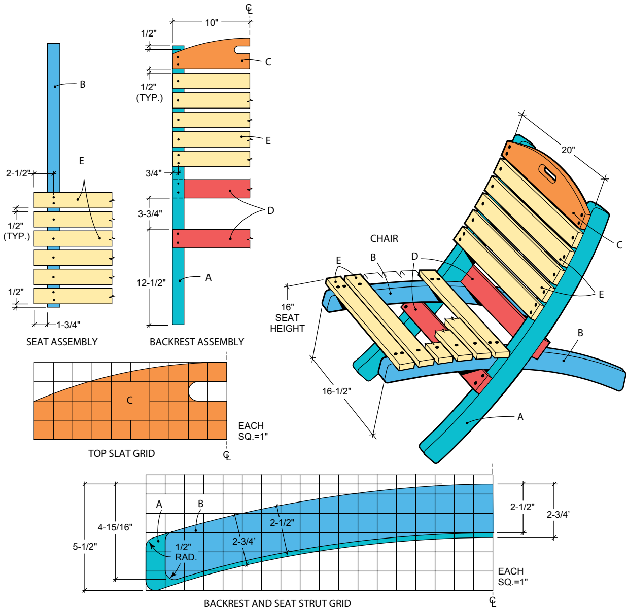
FIG. A PATIO CHAIR DETAILS
