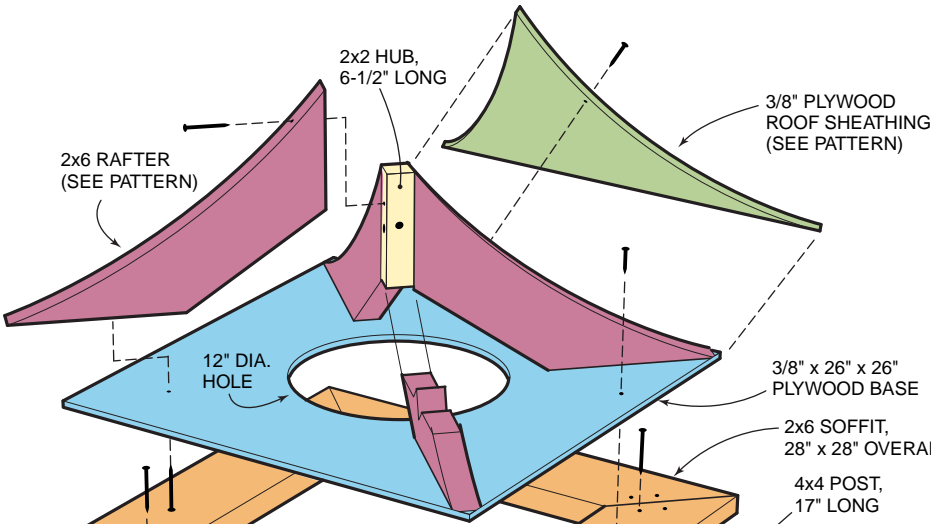
Fig. A Cupola Details
