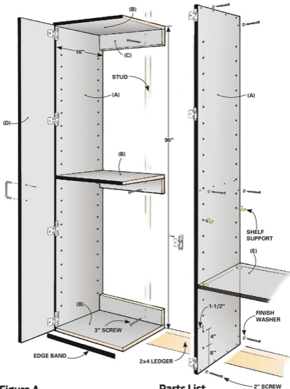
Figure A Upright cabinet construction
