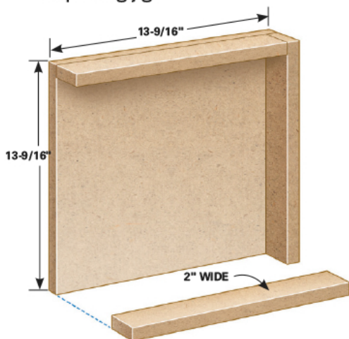
Figure C Squaring jig
