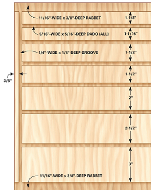
Figure B Side detail
