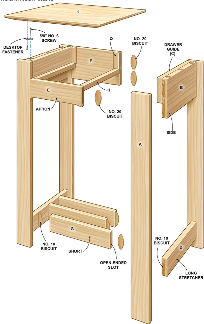
Figure A Mackintosh table
