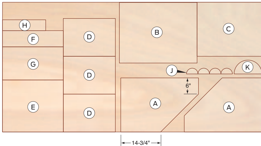
Figure B Plywood cutting diagram
