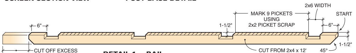
DETAIL 1 - RAIL
