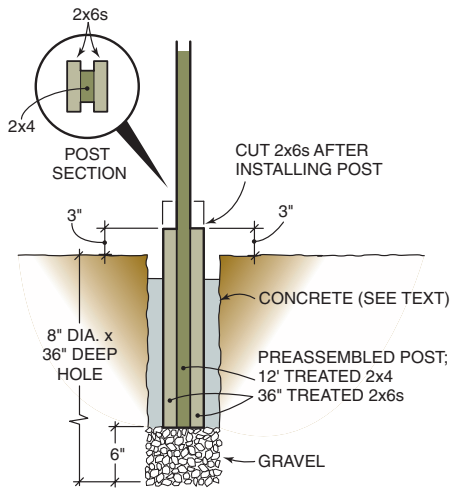
POST BASE DETAIL
