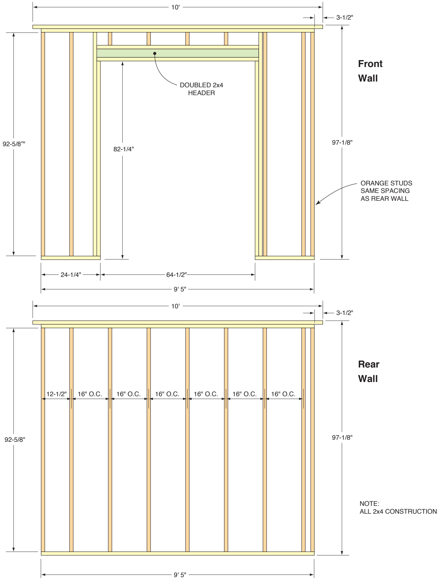
Figure E Front & Rear Walls Framing
