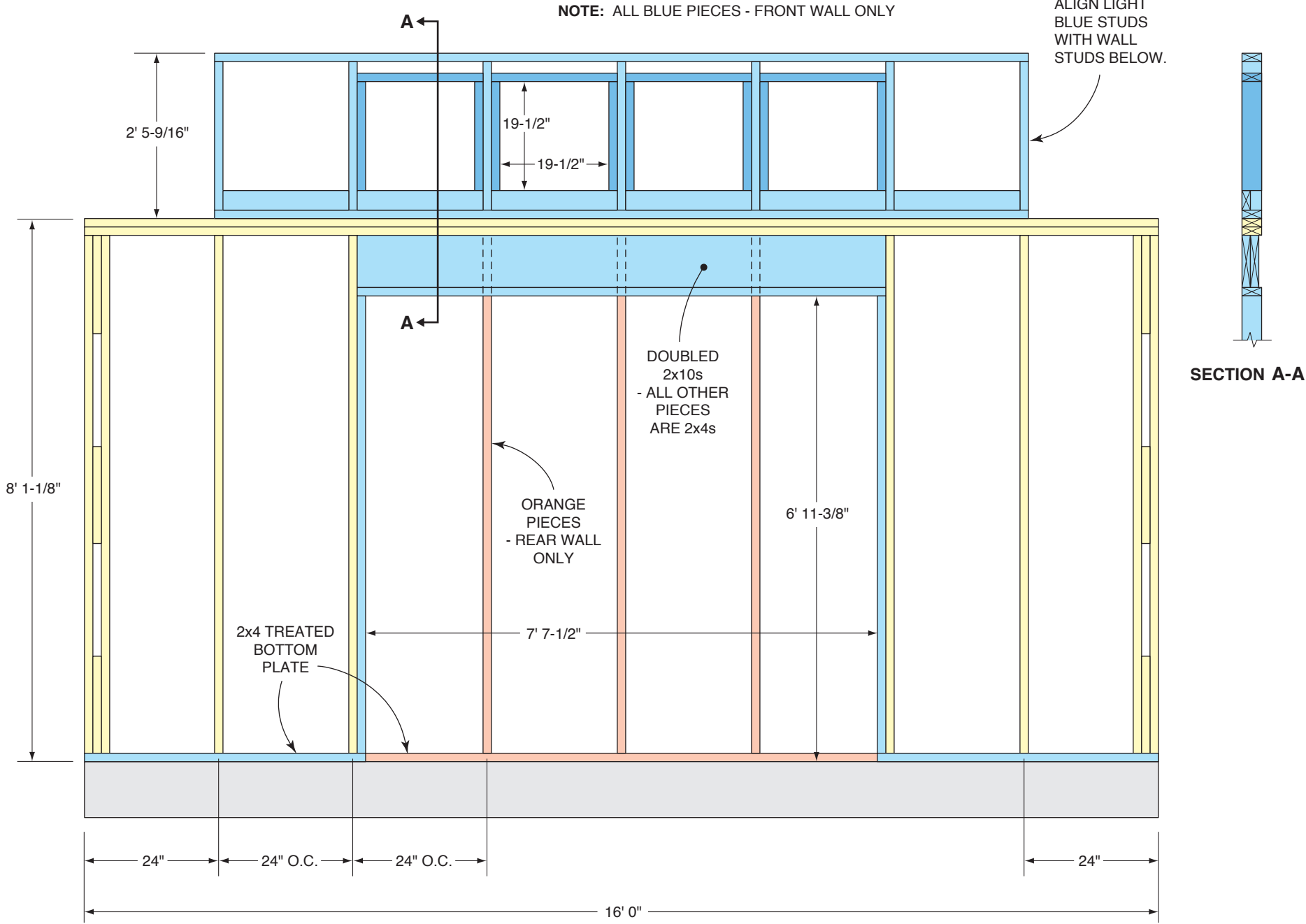
Figure D Front & Rear Wall Framing
