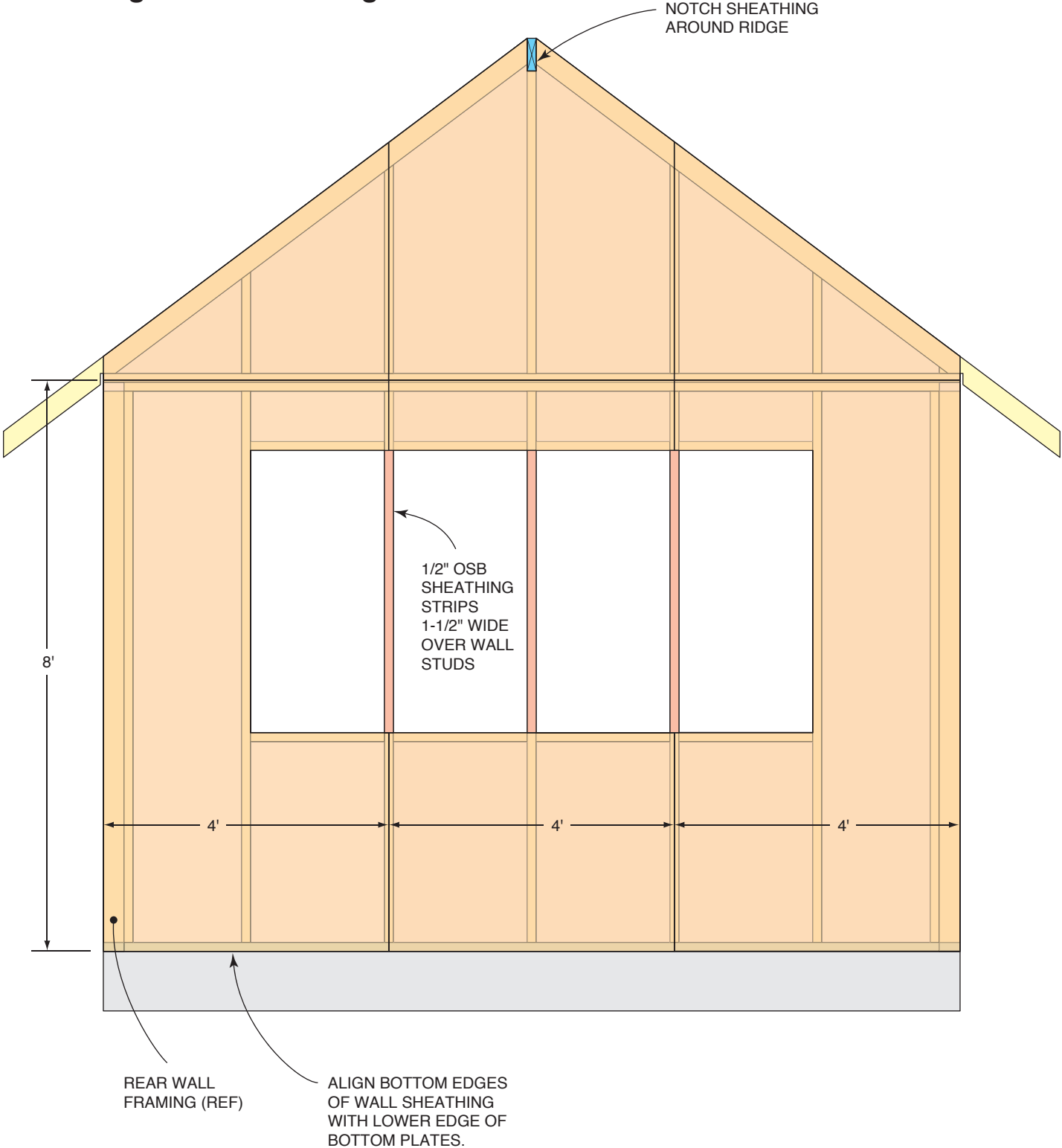
Figure E Left & Right Wall Sheathing
