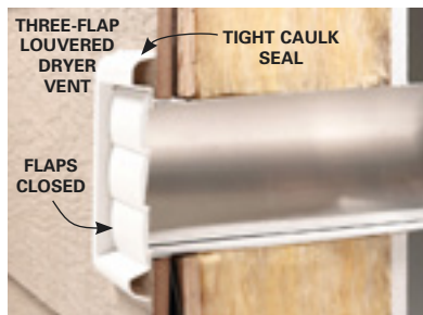
The vent flaps are completely closed and the flange is caulked to stop air infiltration.
