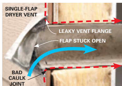
Check that the flap (or flaps) is closed, the vent is flush against the house, and the area around the vent is properly caulked.
